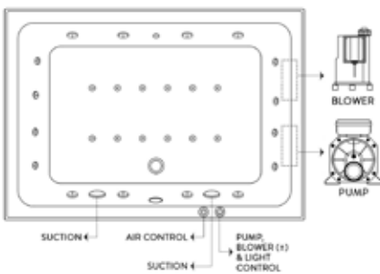
System 8ESF - Deluxe SPA 8 Self-Draining Super Flat Whirlpool Jets, Electronic Control Switch, 4 Back & 4 Feet Jets, Underwater Lighting, 12 SPA Air Jets
