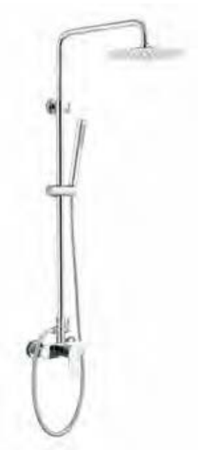
Conrad Shower Column with Shower Head Dia. 200 mm with Single Function Hand Shower & Hose Height Adjustable 850-1200 mm Min. Operating Pressure 1.5 bar MP
