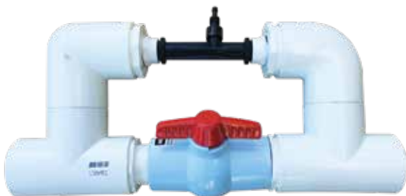
Venturi Manifold
