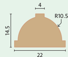
QW-SDA3 4mm Glazing Bar £6.91
