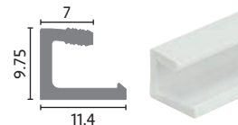
QW-GCA-75 or QW-GCA Glazing Bead Clip
