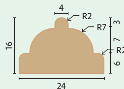
QW-SDA2 3mm Glazing Bar £10.46
