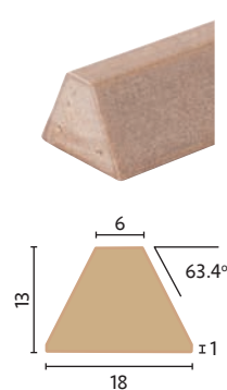
QW-BB4 6mm Glazing Bar £6.18
