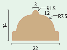
QW-SDA1 3mm Glazing Bar £7.12
