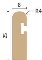
QW-PB8 8mm Parting Bead £6.48
