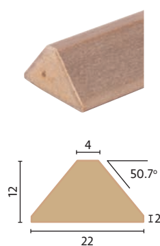
QW-BB3 4mm Glazing Bar £6.18
