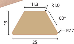
QW-BB6 11.3mm Georgian Bar £9.80
