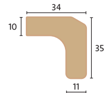
QW-SD-HD1 Head Drip
