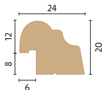
QW-DGB1 Door Glazing Bead
