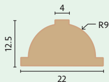
QW-OB1 4mm Glazing Bar £6.91
