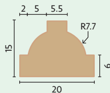
QW-OB2 2.5mm Glazing Bar £6.98
