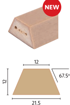
QW-BB1 12mm Glazing Bar £6.25
