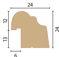
QW-DGB2 Door Glazing Bead
