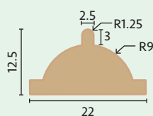
QW-OB2 2.5mm Glazing Bar £6.98
