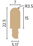
QW-CPB7-NI 7mm Parting Bead £7.57
