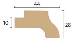
QW-HDB1 Head Drip
