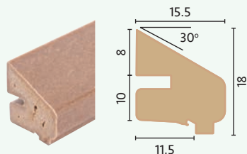
QW-SD3 Glazing Bead
