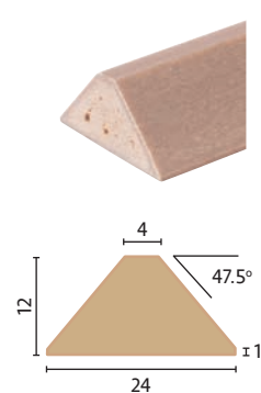
QW-BB5 4mm Glazing Bar £6.80
