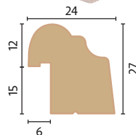
QW-DGB3 Door Glazing Bead
