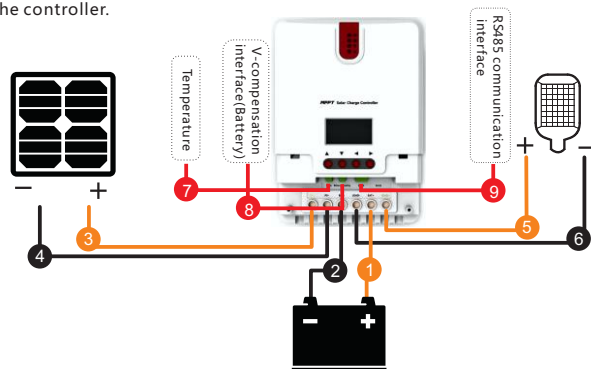
Fig. 2.3 Wiring sequence
