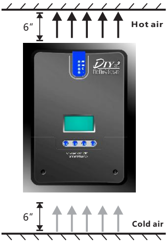
Fig. 2.1 Installation and heat dissipation
