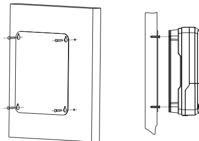
Fig. 2.2 Wall mounting the controller
