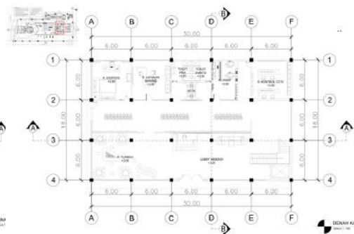
DENAH LT. 1
