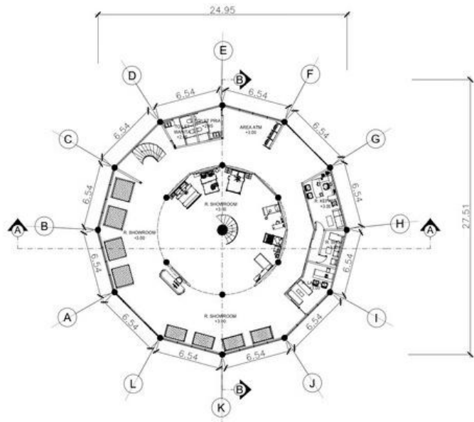
DENAHT. 1
