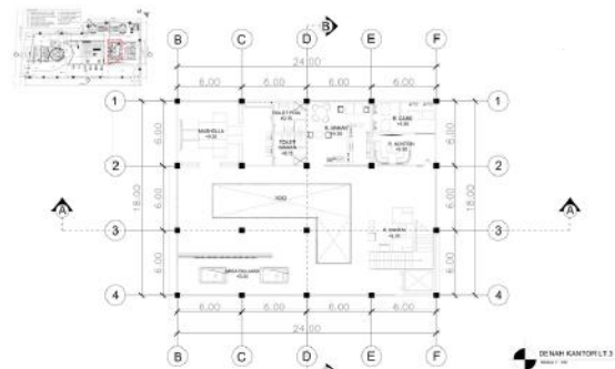
DENAH LT. 3
