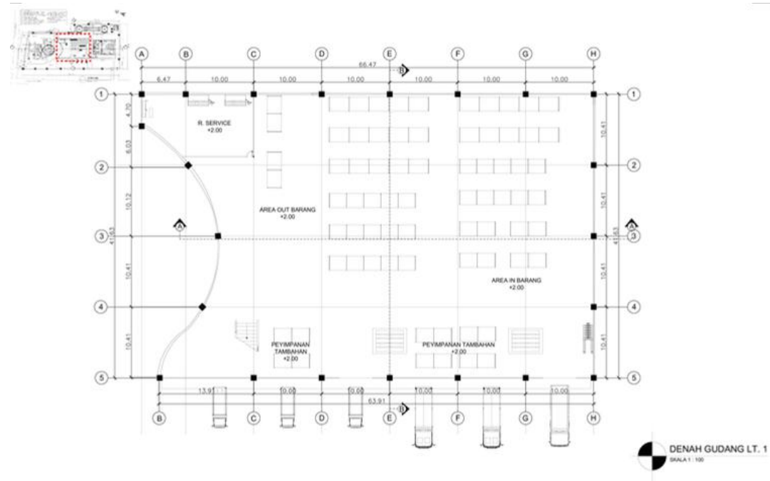
DENAH LT. 1
