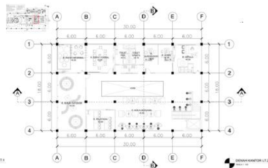
DENAH LT. 2
