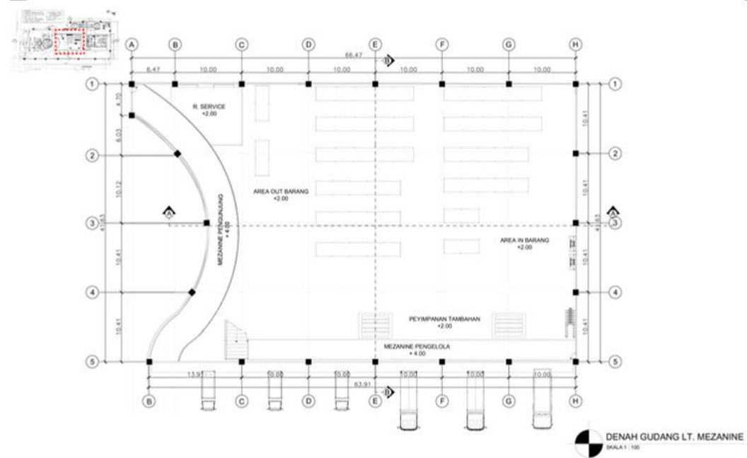
DENAH LT. 2
