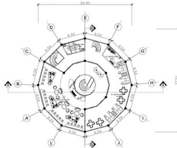
DENAHT. 2
