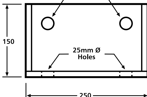
M24 Threaded Holes
