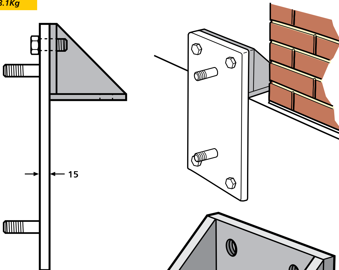
SP ANGLE BRACKET
