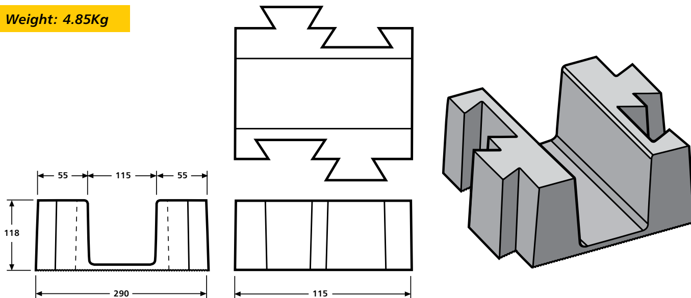
HR4MOD x 2 + Middle Section Assembly
