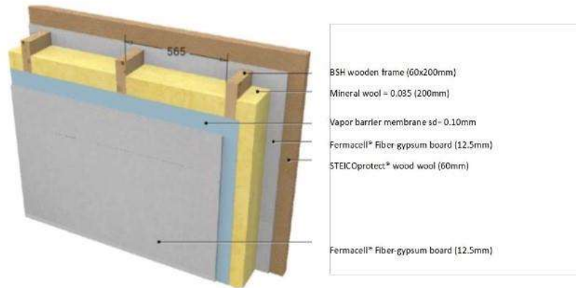
Fig. 6) Typical layout of the external wall layers
