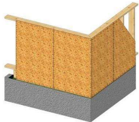
(Fig. 2) Exterior wall sheathing
