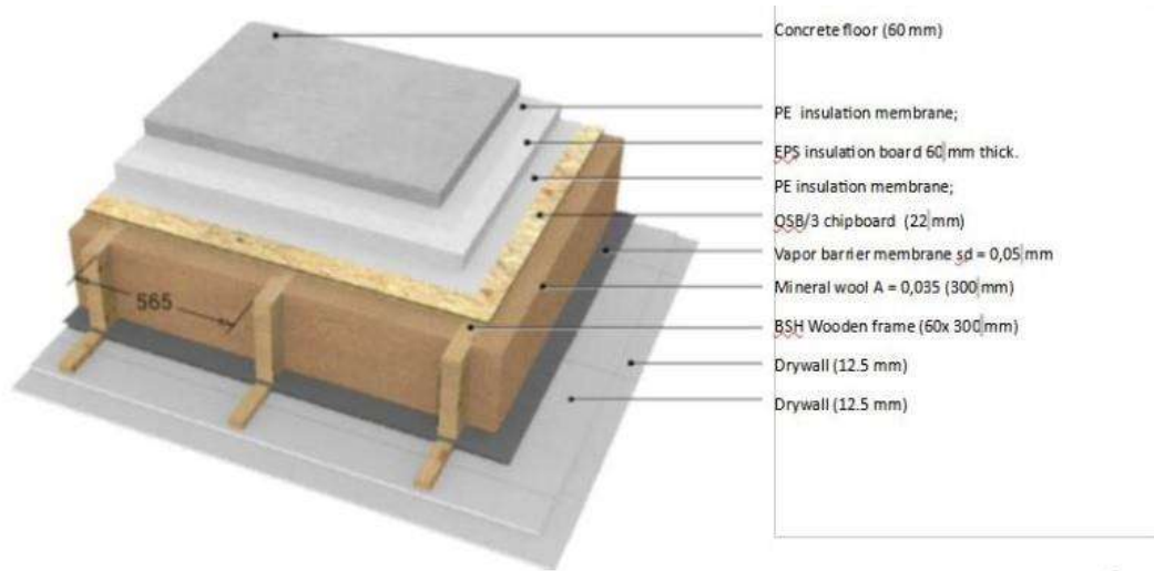
(Fig. 4) Layout of the inter-storey ceiling layers
