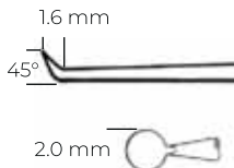
SHEEHY MCK 06.104.99 straight shaft / düz şaft 16 mm
