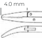
RICHARDS MCK 06.105.32 curved left / sola eğri straight shaft / düz şaft 8 cm
