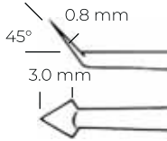
JORDAN MCK 06.103.46 straight shaft düz şaft 17.5 cm
