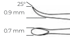
GUILFORD MCK 06.103.47 straight shaft düz şaft 14 cm
