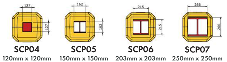
Overall Dimensions 410mm x 410mm x 1045mm High
