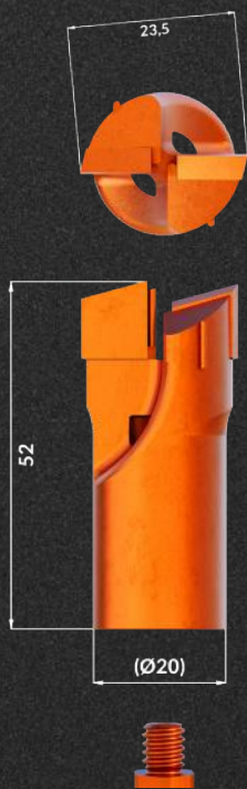
16MM THREAD
