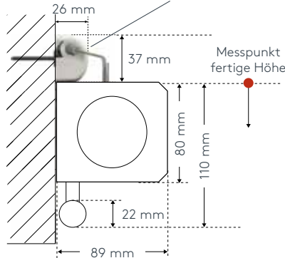
Wandmontage W
