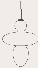
RIZZATTO 43 Dimensions ø400mm x 626mm Options satin brass / opal or satin silver / opal Cable colour gold or silver fabric Cable Length max 4000mm Light source E27
