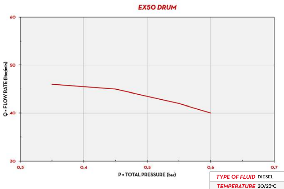
2" CONNECTOR
