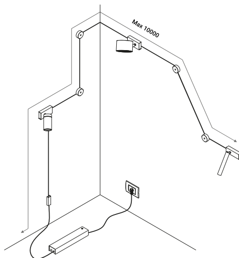
Example of combined installation between various devices with driver with plug
