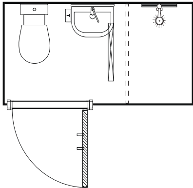
Single Bathroom Layouts
