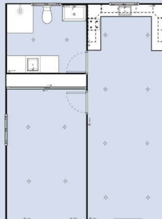
1 Bed Layout
