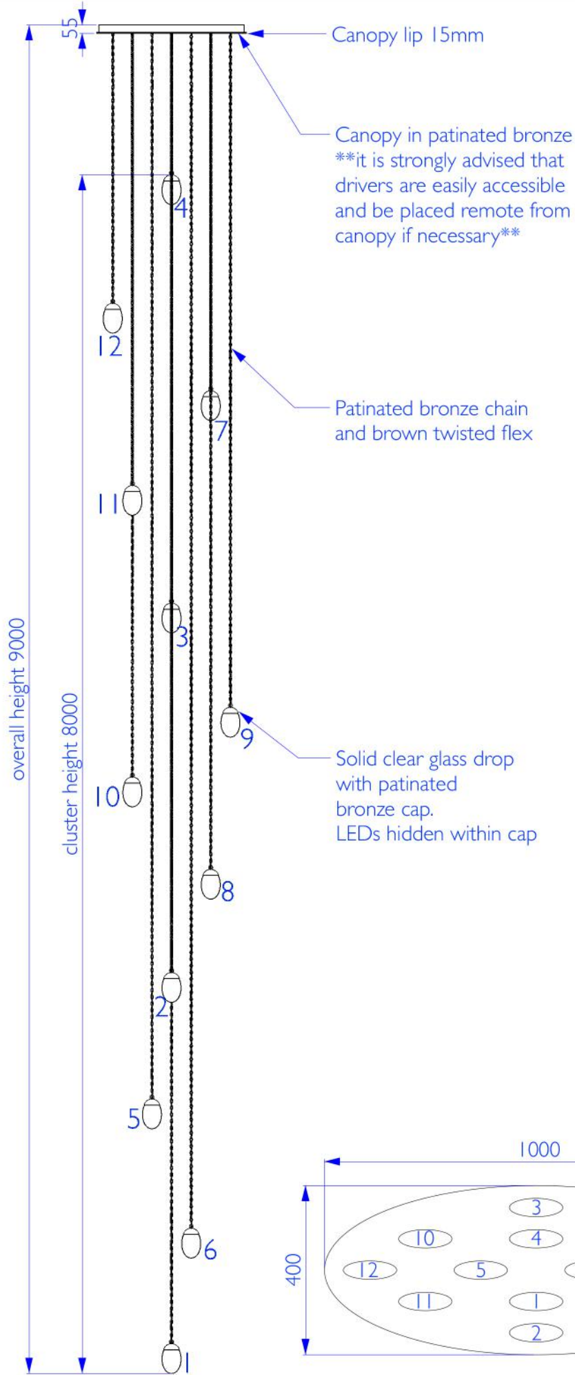
TOP VIEW
