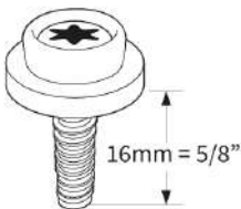
SELF TAPPING SCREW STUD 5/8
