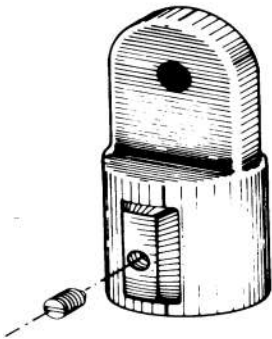
EYE END
