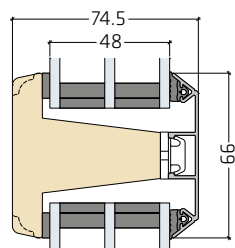
60 mm sprosse | NATic12-61L48
