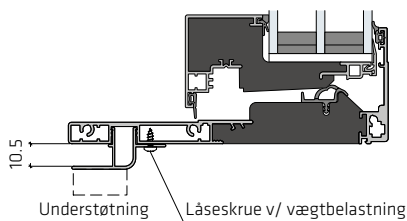
10 mm not | PLU-NOT007
