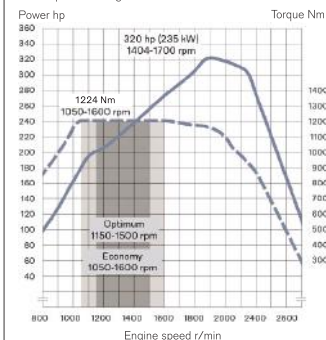
ENGINE D8K320-EU6SCR
