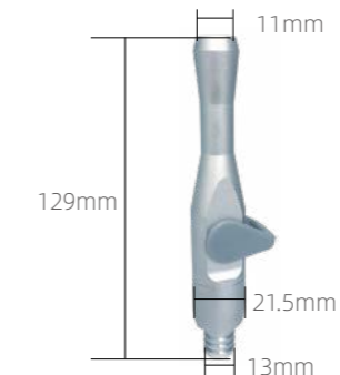
分体式强吸手柄 Strong Suction (split type) 30-07
