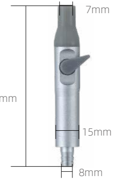
弱吸手柄(硅胶头) Weak Suction (silicone nozzle) 30-05
