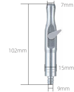
连体式弱吸手柄 Weak Suction (one-piece) 30-04
