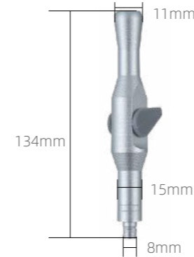
连体式强吸手柄 Strong Suction (one-piece) 30-03
