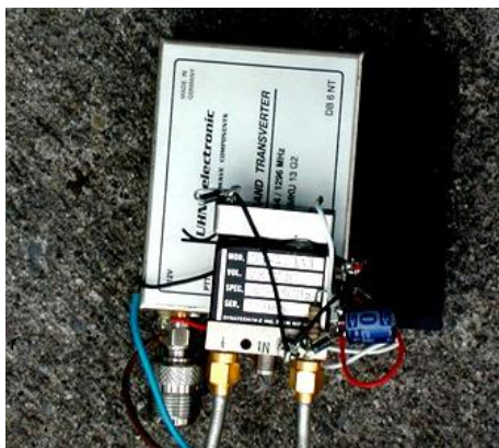
Khune 23cm transverter with 12V coaxial relay
