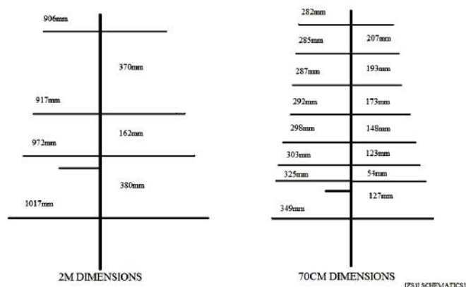
"BOW" AND "ARROW" SATELLITE ANTENNA SCHEMATIC
