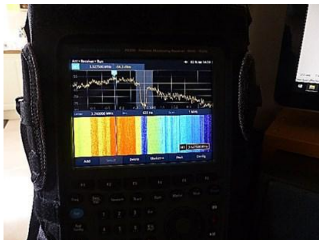
Fig. 4 Spectrum display of interference on the waterfall display of the Rohde Schwarz receiver
