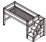
SEMI-HIGH BED WITH STEPLADDER H 128 x W 257 x D 102 Ground clearance below the bed 89 CM
