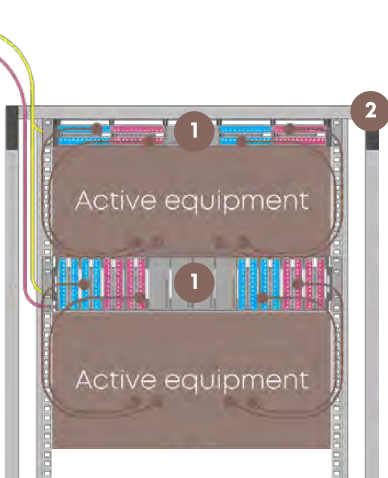
SYLFA HD 19 inch patch panels
