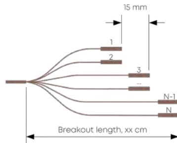
Breakout type 2 #1 on shortest leg
