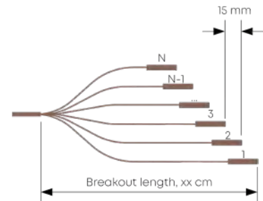
Breakout type 3 #1 on longest leg
