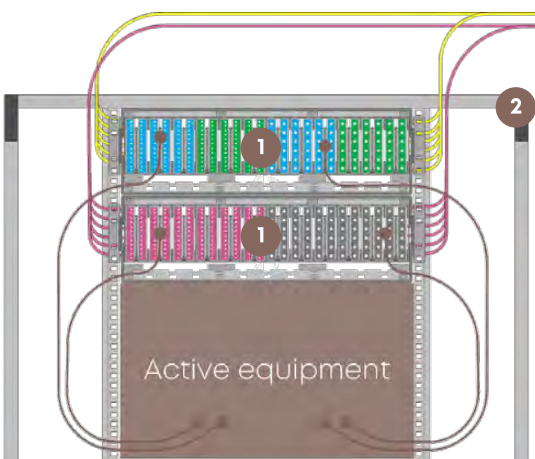
ODF SYLFA HD in 19 inch cabinet
