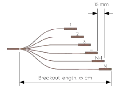
Breakout type 1 #1 on shortest leg
