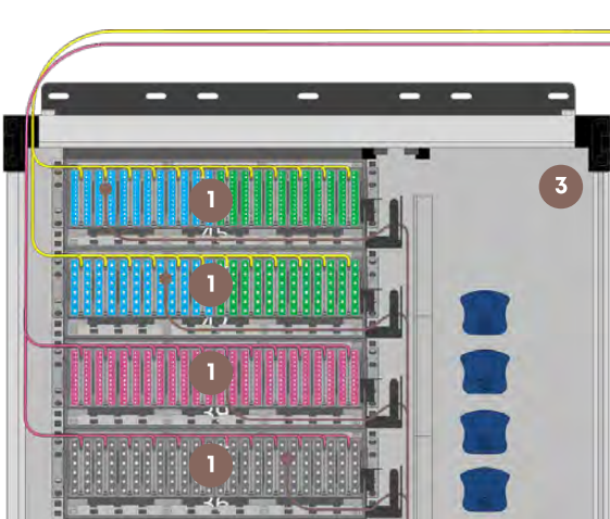
ODF SYLFA HD in 300 mm rack
