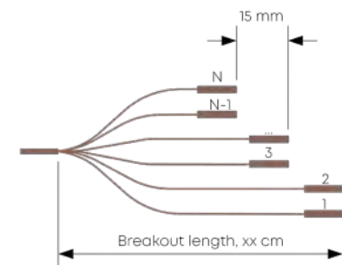
Breakout type 4 #1 on longest leg
