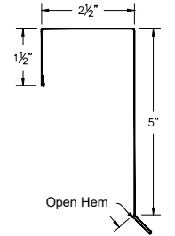
40 ABS Gable Flasing (ABSGFcc)
