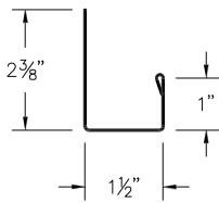
⑤⑤ PBR J Channel (PBRJcc)
