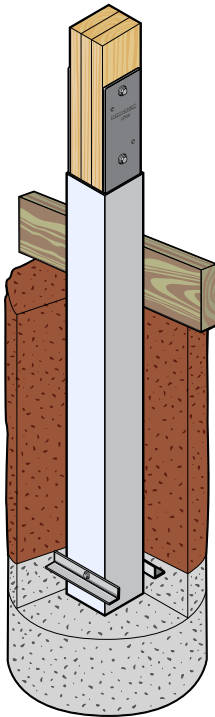
SHOWN WITH UPLIFT HARDWARE (SOLD SEPARATELY)
