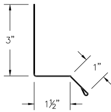
⑤① PBR Drip Cap (PBRDCcc)
