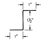
38 ABS Metal "Z" Closure (ABSZcc)
