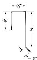
45 ABS Rake Trim (ABSRtcc)
