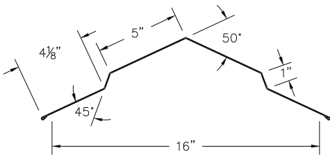
③④ 20" Ridge Cap (CP20cc)
