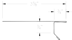
38 ABS Metal "Z" Closure (ABSZcc)
