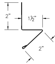
⑤④ PBR Base Angle (PBRBAcc)
