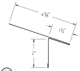
35 ABS Residential Eave (ABSREcc)
