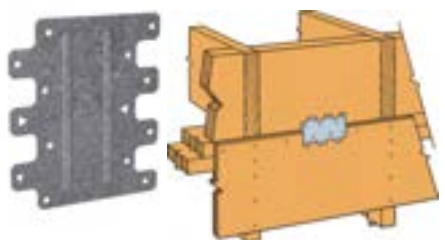
HEAVY TIE PLATE
