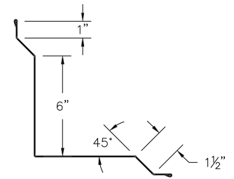
⑤⑧ PBR Inside Corner (PBRICcc)
