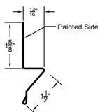
Base Angle BAcc • 10' 2"
