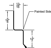
Double Angle DAcc • 10' 2"
