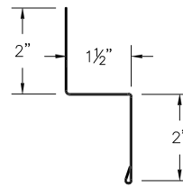
⑤③ PBR Double Angle (PBRDAcc)
