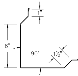
⑤⑥ PBR Outside Corner (PBRRCcc)
