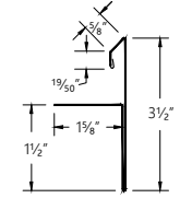
50 ABS Slim Line Rake (ABSSLRcc)
