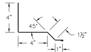
⑤② PBR Universal Sidewall (PBRSWcc)
