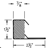
12 ABS Vented "Z" Closure (ABSZVcc)
