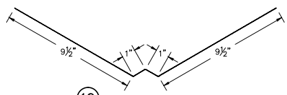
19 ABS W Valley (ABSWVcc)
