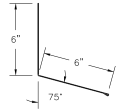
①① Universal Endwall (PBREWcc)
