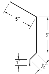
⑤⑦ PBR Fascia Trim (PBRFTcc)
