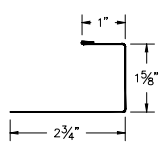
39 ABS Starter "J" (ABSSJcc)
