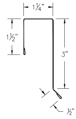
45 ABS Rake Trim (ABSRtcc)
