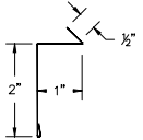
43 ABS Counter Flashing (ABSCFcc)
