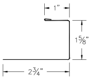
39 ABS Starter "J" (ABSSJcc)
