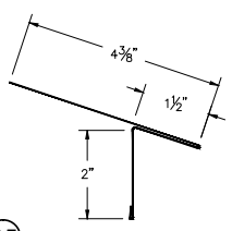
35 ABS Residential Eave (ABSREcc)
