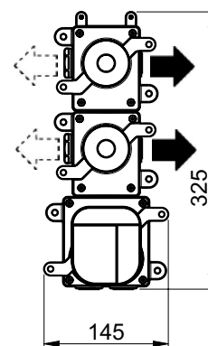
E176002 BUILT-IN THERMOSTATIC 2 WAY
