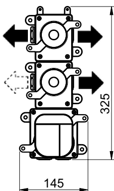
E176303 BUILT-IN THERMOSTATIC DIVERTER 3 WAY
