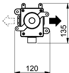
E175501 SHUTOFF VALVE BUILT-IN MODULE
