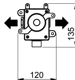
E179502 DIVERTER BUILT-IN MODULE
