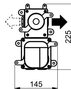
E176001 BUILT-IN THERMOSTATIC 1 WAY
