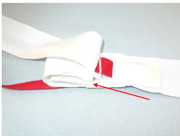
Stow the Spectra Line Loop into the looped polyester sleeve opposite the long pin channel.
