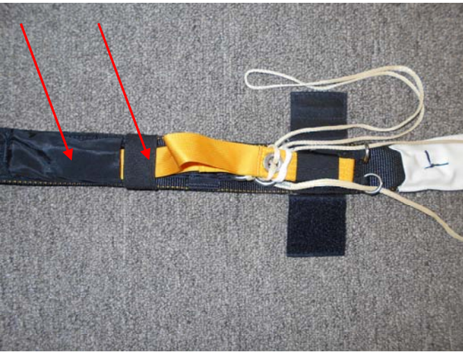
Tuck the Toggle into the sleeve shown and bring up the Elastic Retainer over the Toggle.
