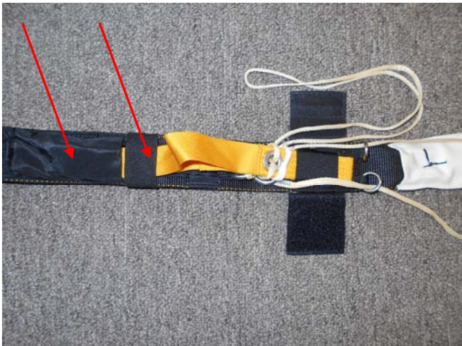
Tuck the Toggle into the sleeve shown and bring up the Elastic Retainer over the Toggle.
