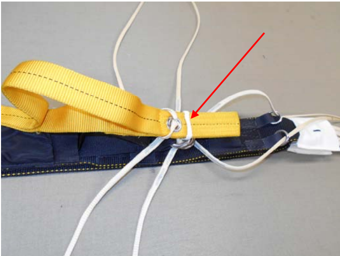
Pass the tip of the Main Toggle through the Spectra Loop as shown.
