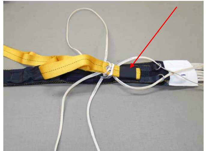
Tuck the Toggle into the 1 1/2" T-III Retainer.
