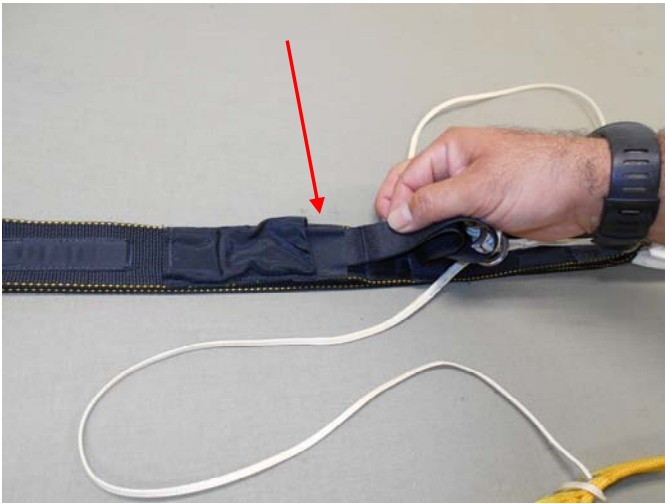
Stow the Flaring Toggle into the 1 1/2" T-III pocket.
