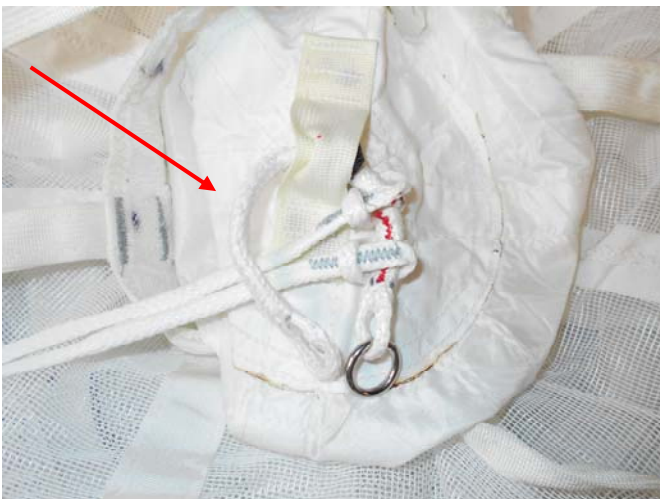
Remove the Soft Link.
