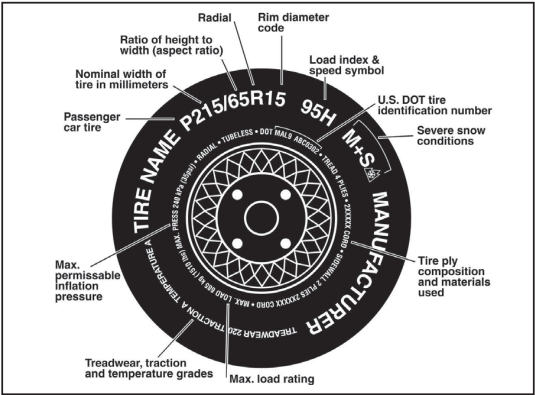
Figure 3: Typical Passenger Tire Markings
