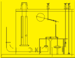
CONTROL GEAR SYSTEM FOR RAPID GRAVITY FILTER PLANT
