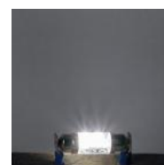
Part No. 201F3632VW – White Part No. 201F3632VR – Red FESTOON LED 10X36MM Multivolt 24-32V, set of 2pc € 12,00 excl. VAT / € 14,52 incl. VAT
