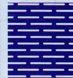
48 1 x 13 .039" x .512" -17.8% open
