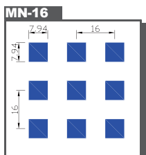
MN-16 Hole size : Q.S. 5.0x5.0mm Pitch : 15.0mm Open Area : 24.63%
