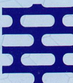
38 6.5 x 20 .256" x .787" -41.2% open
