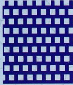
67 3 x 5P 36% open .118" square .197" centers,
