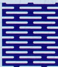
51 1.5 x 15 .059" x .591" -33.3% open
