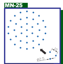
MN-25 Hole size : Dia. 2.5mm Pitch : 10.0mm Open Area : 5.0%
