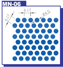
MN-06 Hole size : Dia. 4.5mm Pitch : 6.17mm Open Area : 48.24%
