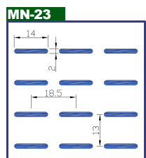
MN-23 Hole size : Olong 2.0x14.0mm Pitch : 13.0x18.5mm Open Area : 11.26%
