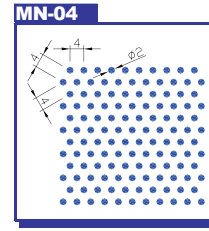
MN-04 Hole size : Dia. 2.0mm Pitch : 4.0mm Open Area : 22.66%
