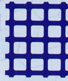
75 7 x 10P 49% open .276" square .394" centers,
