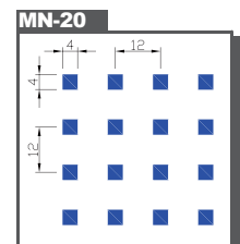
MN-20 Hole size : Q.S. 4.0x4.0mm Pitch : 12.0mm Open Area : 11.11%
