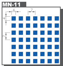
MN-11 Hole size : Q.S. 4.0x4.0mm Pitch : 7.0x7.0mm Open Area : 32.65%
