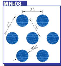
MN-08 Hole size : Dia. 12.0mm Pitch : 20.0mm Open Area : 32.63%
