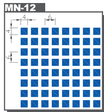
MN-12 Hole size : Q.S. 4.0x4.0mm Pitch : 6.0x6.0mm Open Area : 44.44%
