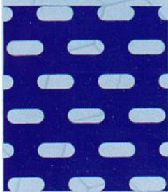
31 4 x 10 .157" x .394" -30.7% open
