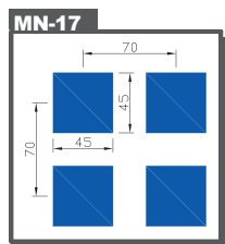
MN-17 Hole size : Q.S. 45.0x45.0mm Pitch : 70.0x70.0mm Open Area : 41.33%
