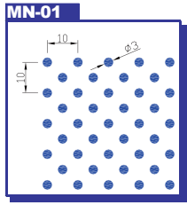
MN-01 Hole size : Dia. 3.0mm Pitch : 10.0mm Open Area : 14%
