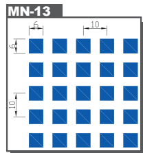
MN-13 Hole size : Q.S. 6.0x6.0mm Pitch : 10.0x10.0mm Open Area : 36.0%
