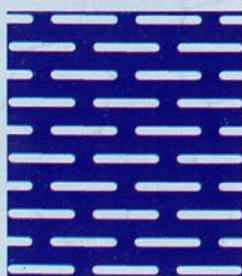
50 1.5 x 11 .059" x .433" -23.1% open
