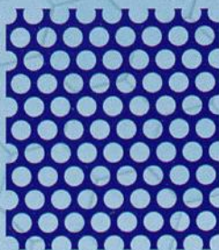
26 3.5 \phi x 5P .1378" diameter .197" centers, 44.4% open
