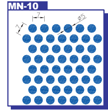
MN-10 Hole size : Dia. 5.0mm Pitch : 7.0mm Open Area : 46.26%
