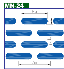
MN-24 Hole size : Olong 5.0x25.0mm Pitch : 11.0x30.0mm Open Area : 39.52%
