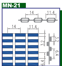
MN-21 Hole size : Olong 3.2x11.4mm Pitch : 6.4x14mm Open Area : 40.71%
