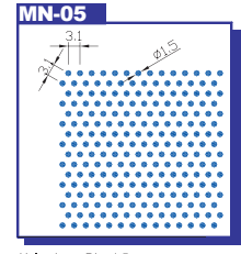
MN-05 Hole size : Dia. 1.5mm Pitch : 3.1mm Open Area : 21.26%
