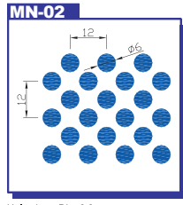
MN-02 Hole size : Dia. 6.0mm Pitch : 12.0mm Open Area : 39.25%
