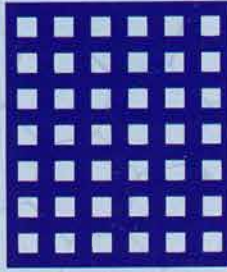
68 3.5 x 6P 34% open .137" square .276" centers,
