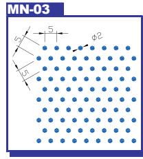
MN-03 Hole size : Dia. 2.0mm Pitch : 5.0mm Open Area : 14.5%
