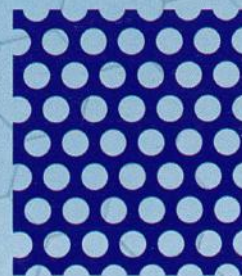
28 4 \phi x 6P .157" diameter .236 centers, 40.2% open
