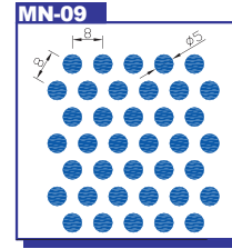
MN-09 Hole size : Dia. 5.0mm Pitch : 8.0mm Open Area : 35.4%
