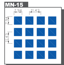
MN-15 Hole size : Q.S. 7.94x7.94mm Pitch : 11.43x11.43mm Open Area : 48.26%
