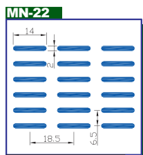
MN-22 Hole size : Olong 2.0x14.0mm Pitch : 6.5x18.5mm Open Area : 22.57%
