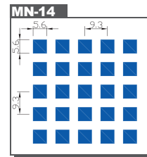
MN-14 Hole size : Q.S. 5.6x5.6mm Pitch : 9.3x9.3mm Open Area : 36.26%
