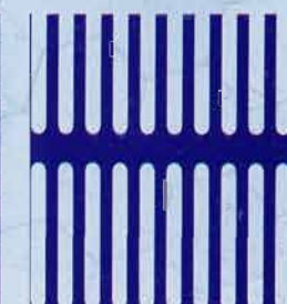
42 2.5 x 24 .098" x .945" -51.2% open
