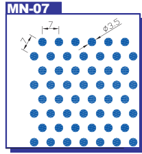
MN-07 Hole size : Dia. 3.5mm Pitch : 7.0mm Open Area : 22.67%
