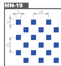
MN-19 Hole size : Q.S. 5.0x5.0mm Pitch : 15.0mm Open Area : 22.22%
