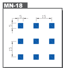
MN-18 Hole size : Q.S. 5.0x5.0mm Pitch : 15.0x15.0mm Open Area : 11.11%
