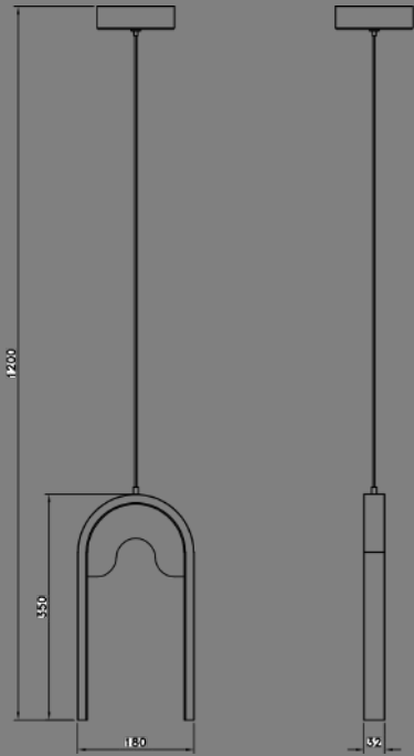
MD23144-1B Lamp Size: L18*W3*H36CM Sand Black/ Sand White, Wood Deco Panel Opal White diffuser, LED 10W, 3000K/4000K
